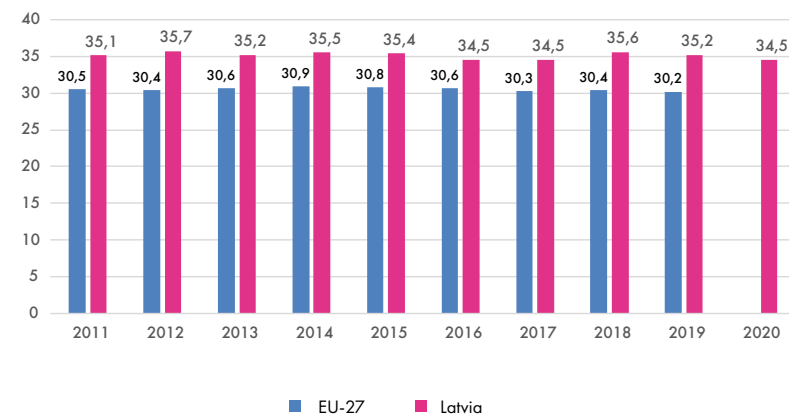
GINI COEFFICIENT
